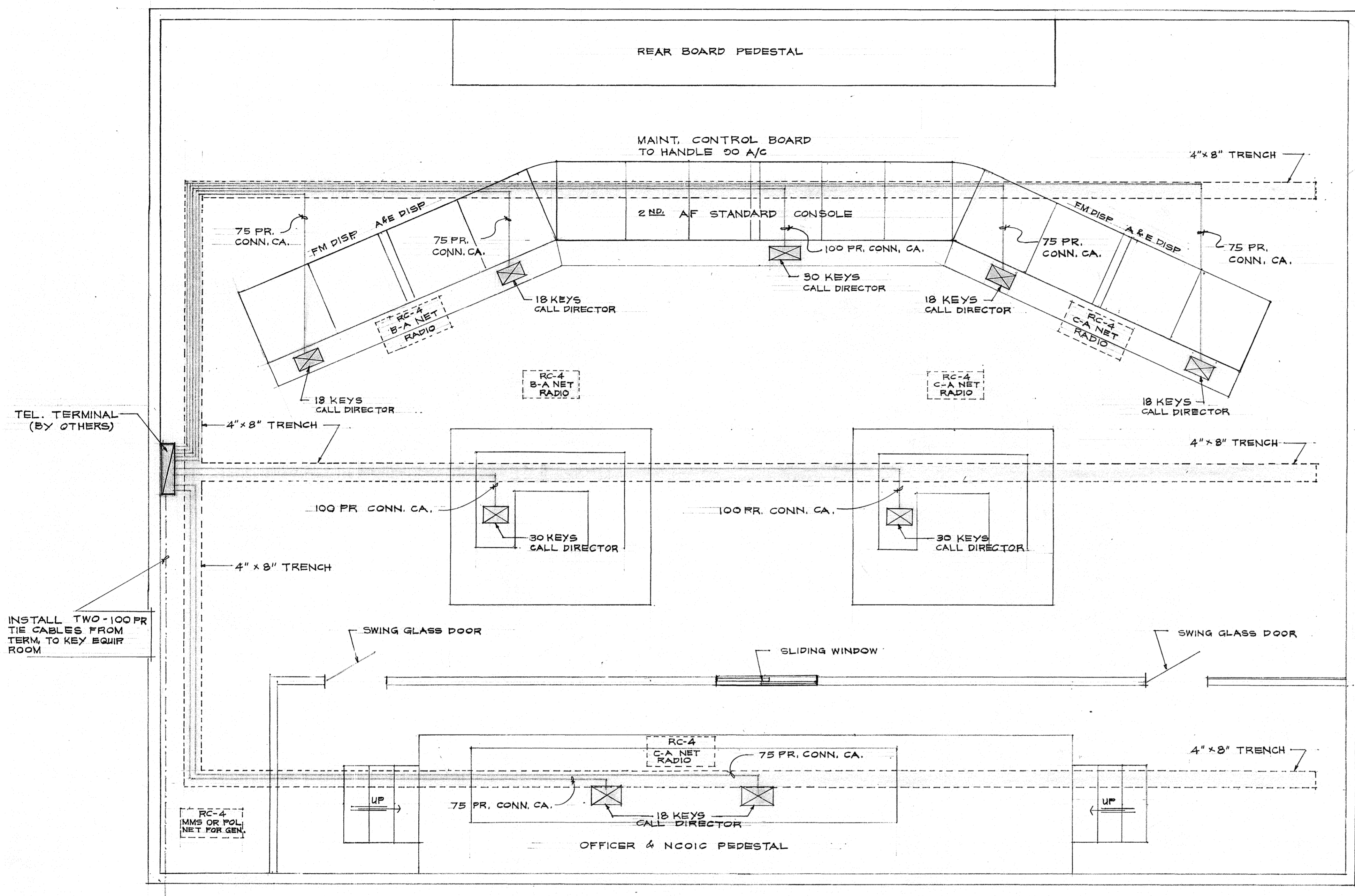
INSTRUMENTS LAYOUT SCALE: NONE
