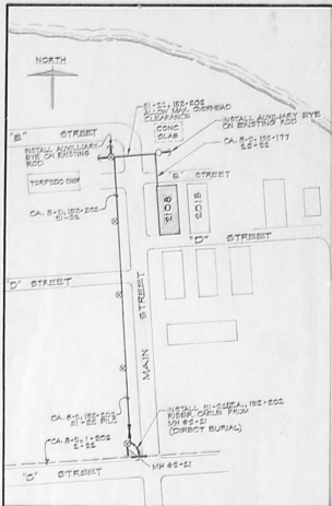
LOCATION PLAN SCALE: 1" = 100'-0"
